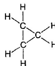
cyclopropane
