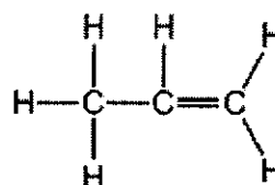
propene
