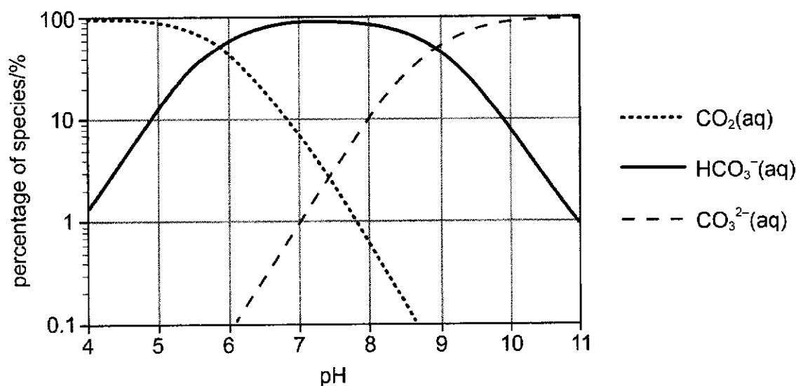
Fig. 8.1: Bjerrum plot
