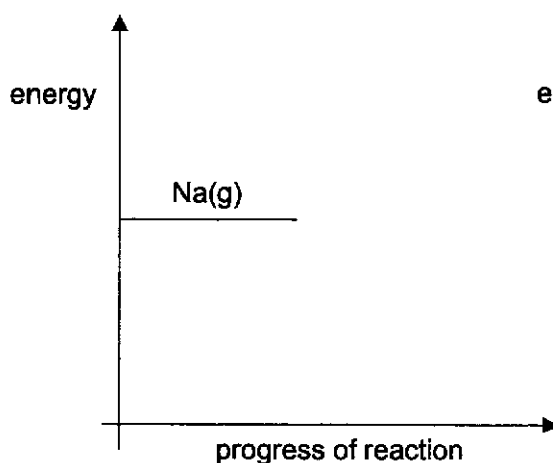
first ionisation energy of sodium
