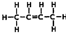
2-butene
