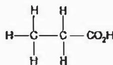
compound C
