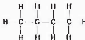
compound F
