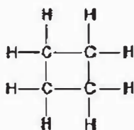
compound A
