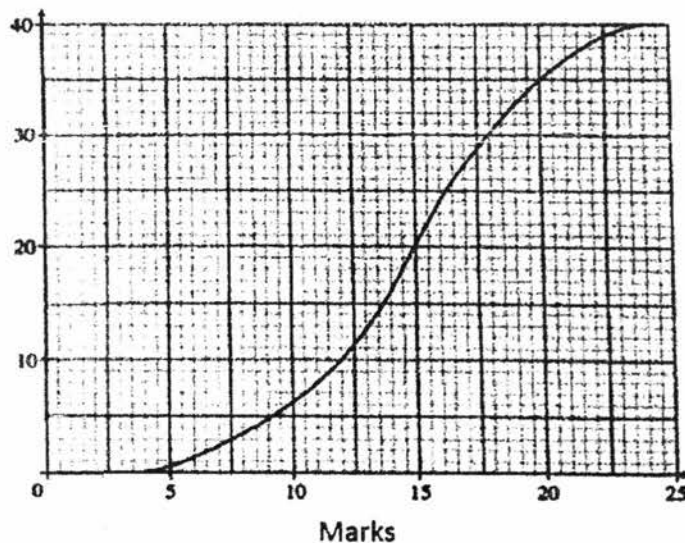
Cumulative Frequency
