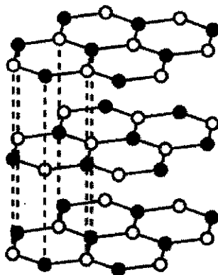
structure X
