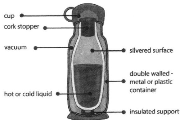
Longitudinal section of traditional vacuum flask
