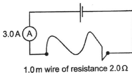
Circuit I
